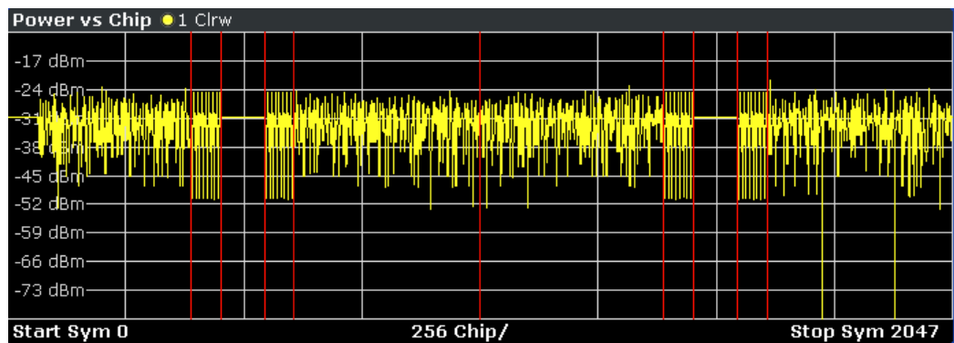
Fig. 4-4: Power vs Chip result display
