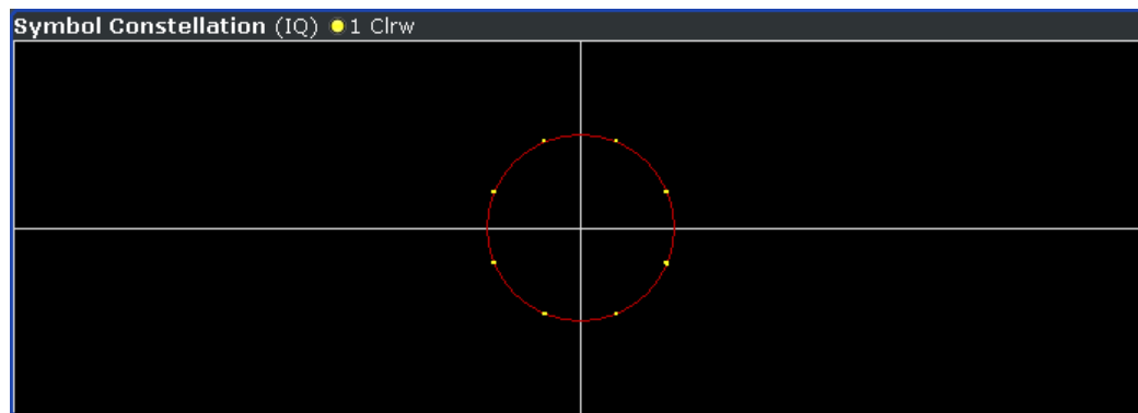
Fig. 4-11: Symbol Constellation result display
